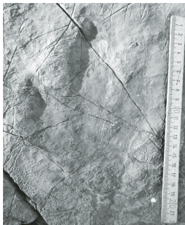
Figure 1. Theropod footprint found at the Vis tracksite
