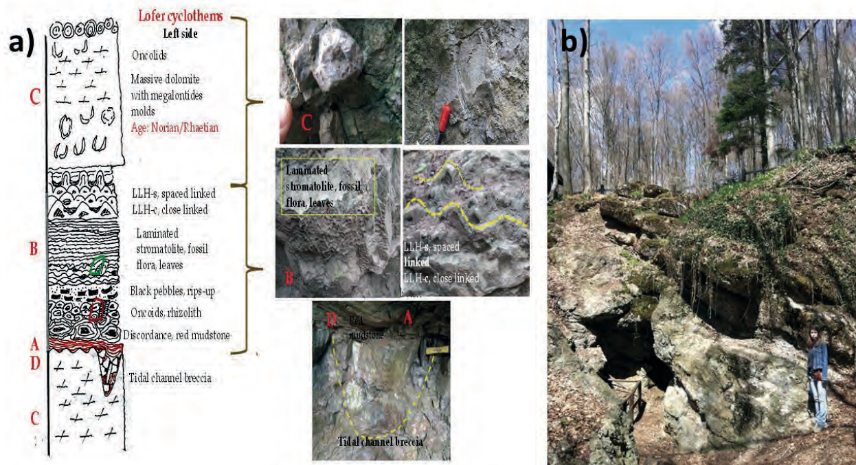
Figure 1. The Lofer cyclothems in the Dachstein dolomite, a. schematic profile, b. in the field
