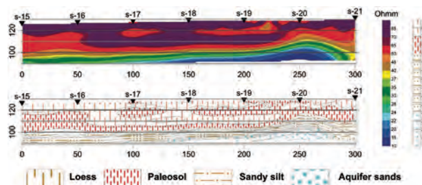
Figure 2. Representative geoelectrical and interpretation profile (sounds: 15 to 21)
